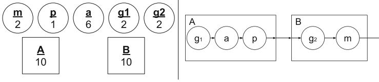
Fig. 2. Given a the set of operations and the sites A and B , Shoal optimizes and places the operations so that the first aggregation is placed on A with the projection reducing network load to the second aggregation operation placed on B .
