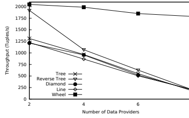
(b) Total throughput for increased load with selectivity .8, two clients per CRNs, and all encryption types used.
