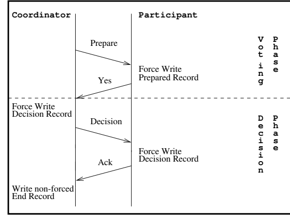
Fig. 7. The basic two-phase commit protocol
