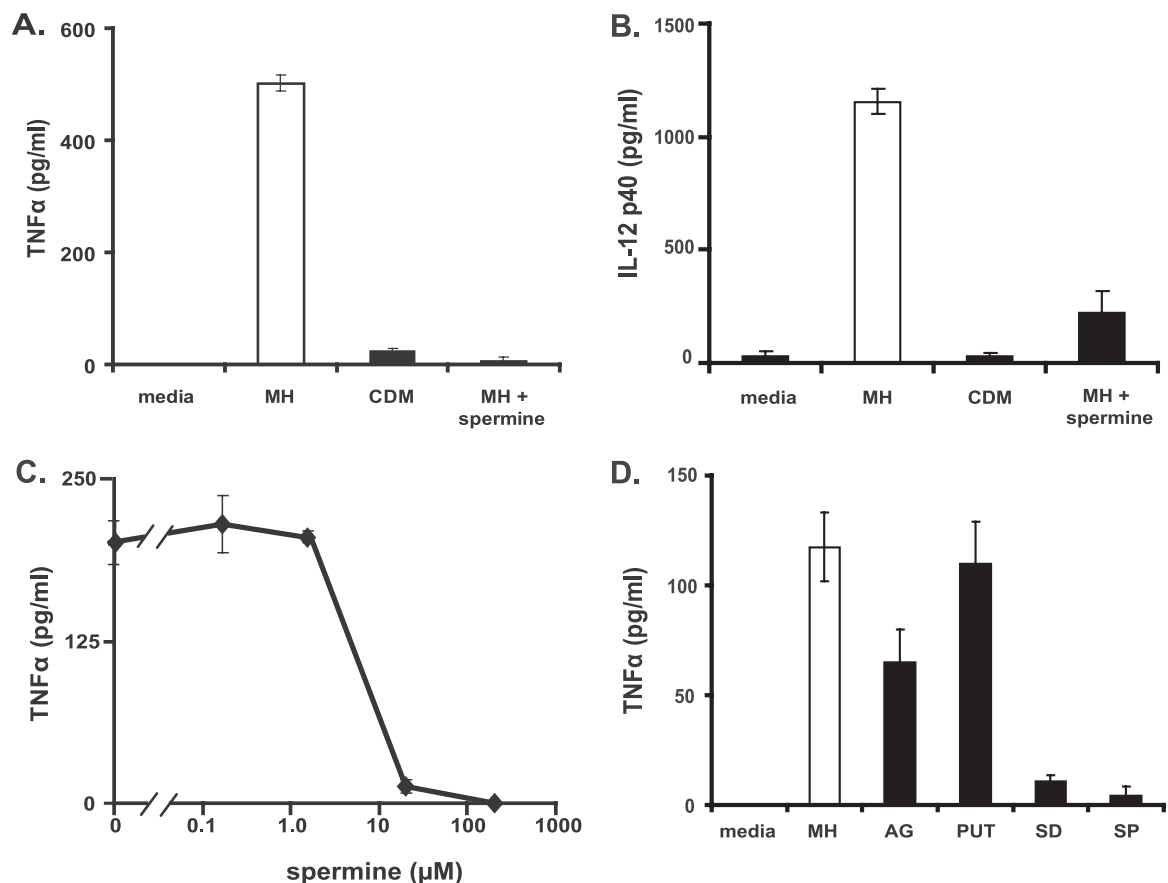
FIG. 1. Inhibition of macrophage cytokine response by Francisella grown in the presence of spermine. (A and B) TNF- \alpha and IL-12 p40 production by human monocyte-derived macrophages following 24 h of culture with F. tularensis LVS grown in the indicated media. Uninfected control wells contained macrophages with no bacteria added (media). Other wells contained macrophages cultured with LVS (MOI, 10) grown in various bacterial media as indicated. CDM contains 200 \mu M spermine; MH broth with spermine was supplemented with 200 \mu M spermine. Data are representative of results from five independent experiments using different blood donors. (C) Titration of spermine levels. F. tularensis LVS was grown overnight in MH broth supplemented with various concentrations of spermine (0, 0.2, 2, 20, and 200 \mu M) before being inoculated into macrophage cultures. Data are representative of results from two independent experiments using different blood donors. (D) Macrophage response to LVS grown in the presence of different polyamines. LVS was grown in MH broth alone or in MH broth supplemented with 200 \mu M agmatine (AG), putrescine (PUT), spermidine (SD), or spermine diphosphate (SP). Macrophages were exposed to bacteria grown in the indicated media at an MOI of 10 for 24 h. Data are representative of results for two independent cultures from two independent experiments. For all panels, TNF- \alpha levels were measured in supernatants by ELISA and data are presented as the means \pm standard deviations of results for triplicate wells within one experiment.
