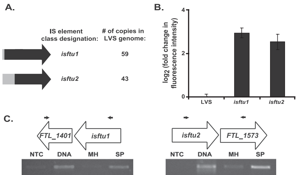
FIG. 3. F. tularensis LVS IS elements contain spermine-responsive promoters. (A) Schematic representation of the two predominant classes of F. tularensis IS elements. Transposase ORFs are indicated by arrows. Light gray boxes represent the conserved sequence found upstream of 10 copies of each element randomly sampled from the genome: ISFtu1 , 30 bp; ISFtu2 , 300 bp. (B) Spermine induces expression of tdTomato using ISFtu1 or ISFtu2 as the promoter element. F. tularensis LVS carrying either ISFtu1 or ISFtu2 (i.e., the transposase gene and 5'-end conserved sequence depicted in panel A) cloned in front of tdTomato was grown in either MH broth or MH broth supplemented with 200 \mu M spermine. Data are presented as means \pm SEM of log 2 -transformed values (normalized fluorescence intensity for culture in MH broth with spermine/normalized fluorescence intensity for culture in MH broth alone) for six independent transformants read in triplicate (18 total measurements per experiment). These data are representative of over 25 F. tularensis LVS transformants harboring each reporter construct. (C) Identification of polycistronic mRNA containing IS elements and downstream genes. Upper panels depict the genomic organization of the IS elements and downstream genes used in this study. Black arrows illustrate the locations of primers used for RT-PCRs. Primers were designed to generate amplicons spanning the IS elements and ORFs in the 3' direction from the IS elements. (Lower panels) Agarose gels stained with ethidium bromide showing amplicons from RT-PCRs. RNA was derived from LVS following growth in broth culture. NTC, no-template control; DNA, positive control using LVS genomic DNA as a template; SP, MH broth with 200 \mu M spermine. No bands were observed in control samples run without RT.
