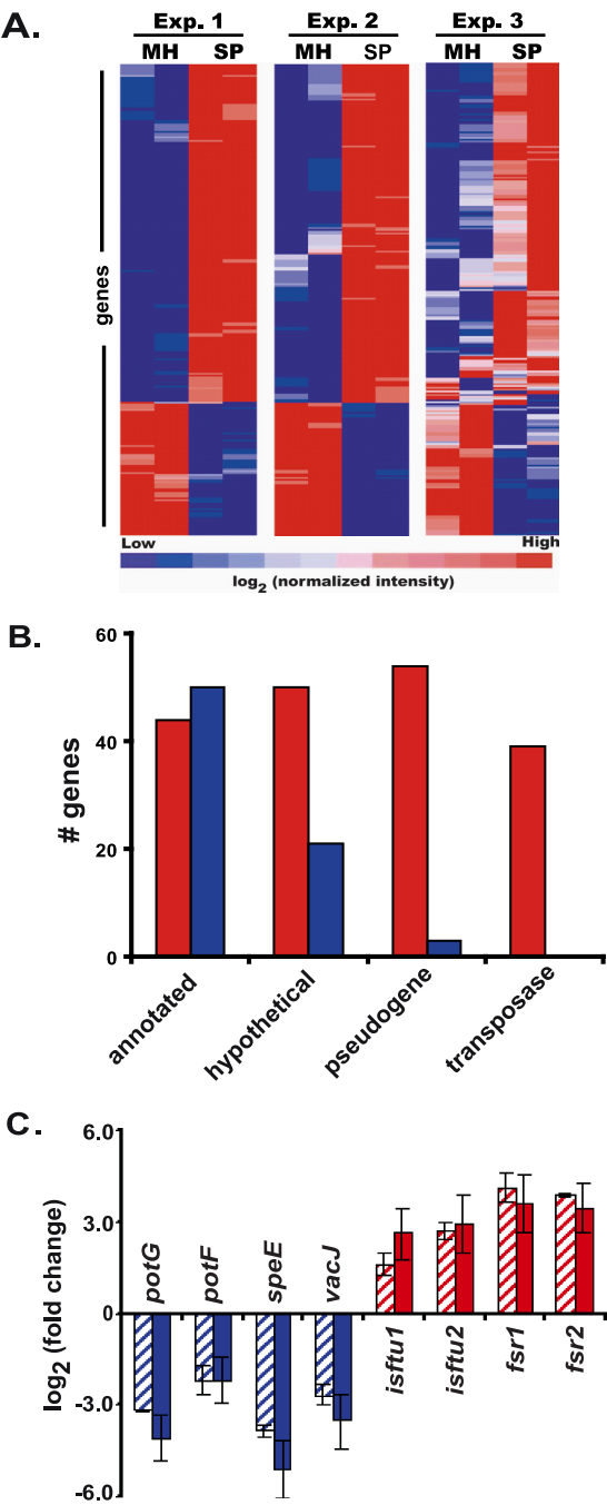
FIG. 2. F. tularensis LVS gene expression changes induced by spermine. (A) Hierarchical clustering of genes identified as statistically significant by the J5 test across three independent microarray experiments (experiments 1 to 3 [exp. 1 to exp. 3]). Fluorescence intensities across each array were normalized by dividing by the median intensity for that array and subjecting the data to \log_2 transformation. The values from each experiment were input into GenePattern individually and clustered using the Pearson correlation. The 185 induced genes and 75 repressed genes clustered together in GenePattern, validating the statistical analysis by the Gene Expression Data Analysis tool. MH, MH broth alone; SP, MH broth supplemented with spermine. (B) Categorical summary of spermine-induced changes in gene expression. Genes exhibiting increased (red bars) or decreased (blue bars) transcription levels were grouped into functional categories based on their NCBI annotation. Category definitions were as follows: annotated genes, those with known or predicted functions; hypothetical genes,
